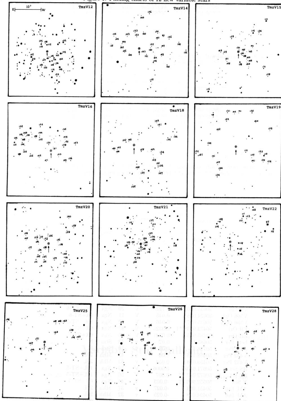
Figure 1. Finding charts of 12 new variable stars
